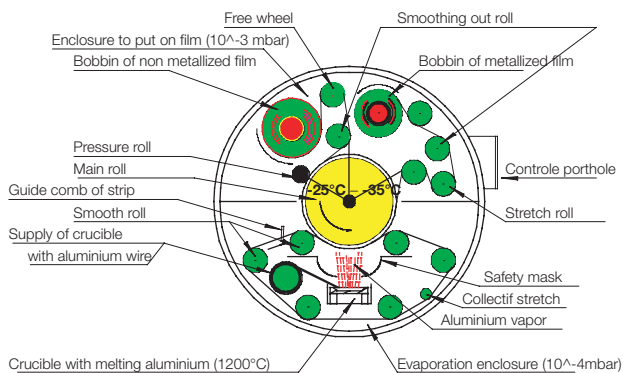
SCHEMATIC DIAGRAM OF THIS EQUIPMENT
