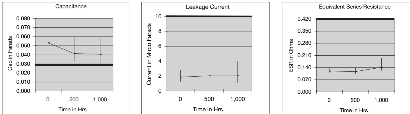
Figure 4: Load Life (rated voltage and max. rated temperature applied)
