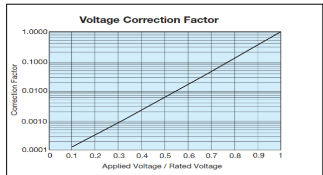
Chart 7: Operating voltage correction factor Fv
