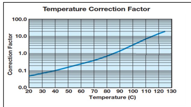
Chart 8: Operating temperature correction Ft
