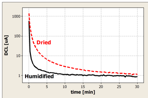
Chart 11. Typical DCL in humid vs dry conditions
