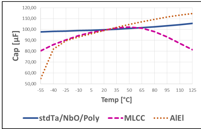
Chart 2: Typical Capacitance Temperature characteristics for different Capacitor technologies
