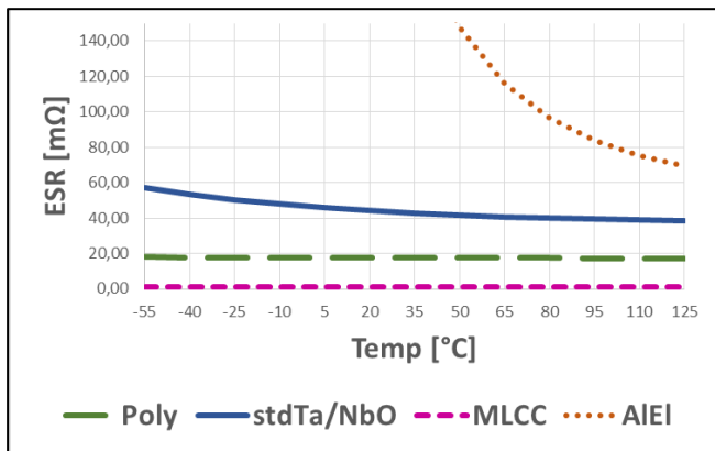
Chart 3: Typical ESR Temperature characteristics for different Capacitor technologies
