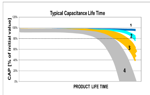
Chart 10. Typical long life time for Capacitance for solid electrolytics
