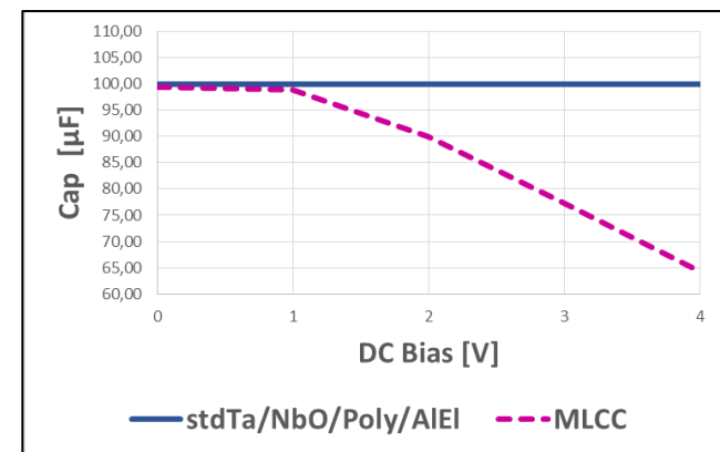
Chart 4: Typical Capacitance DC bias characteristic for different Capacitor technologies
