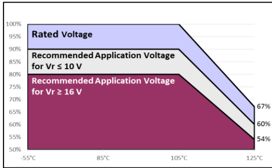
Chart 5: Example of derating chart in datasheet
