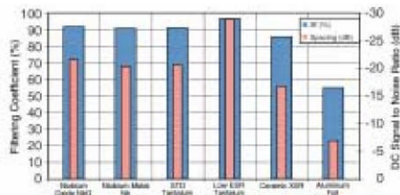
Figure 11, 12. Output ripple voltage and Filtering coefficients comparing different capacitor technologies as the output capacitor.
